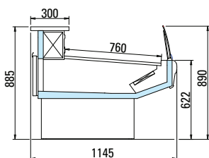
Ventilato/Ventilated SELF
