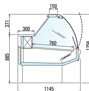
Ventilato/Ventilated VCB
